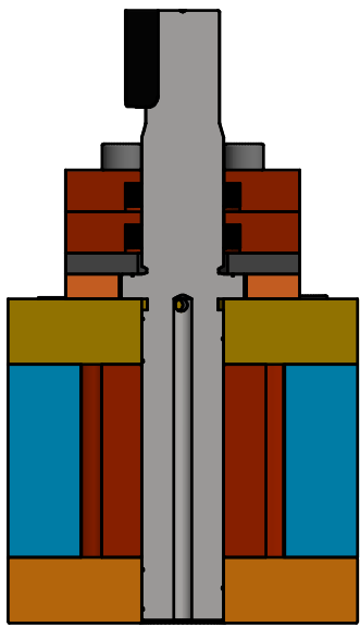
SECTION C-C SCALE 1 / 2
